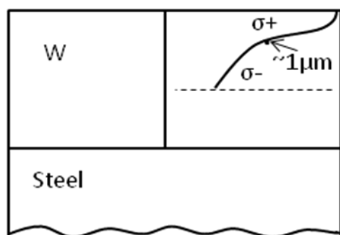
Fig. 6. A scheme of stress distribution over the coating tungsten depth
