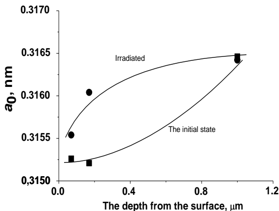
Fig. 3. Distribution of the lattice parameter over the depth of the W coating in the initial state and after hydrogen plasma exposure
