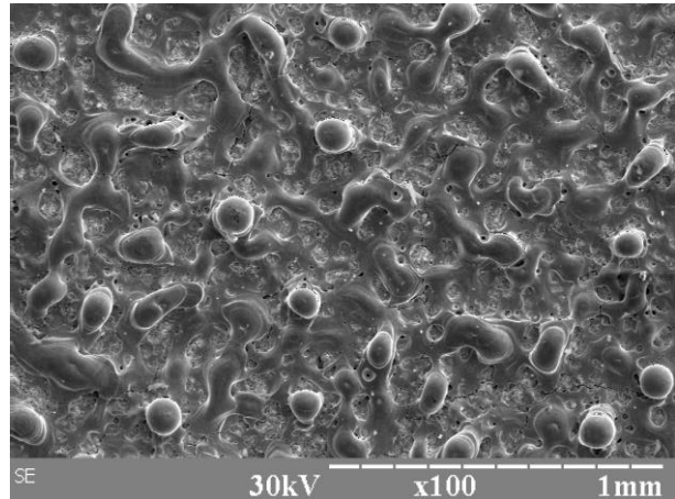
Fig. 4. SEM image of exposed surface
