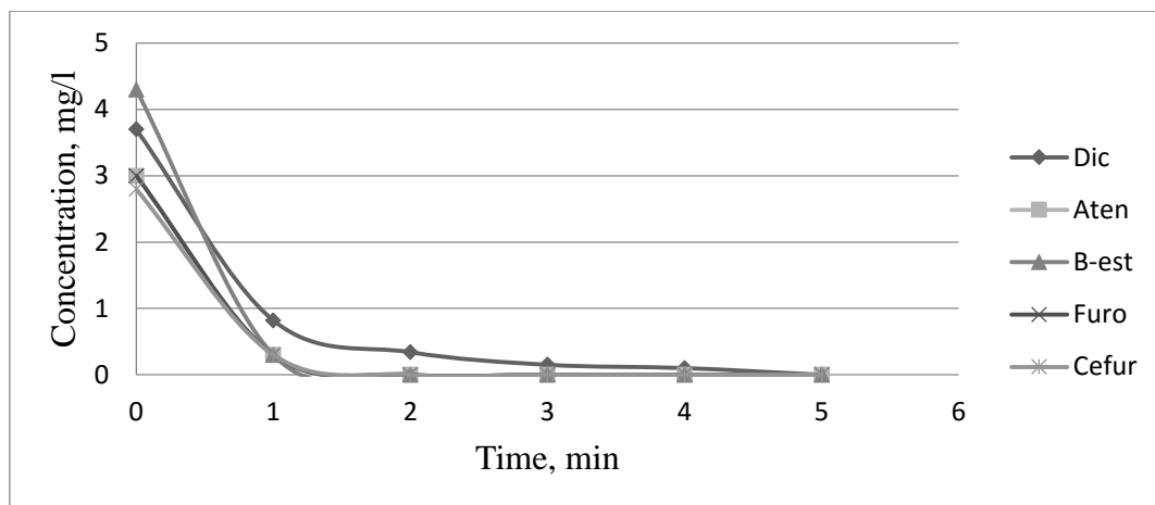
Figure 1. Total kinetic process of PhSb destruction using the RuO 2 anode. Concentration of NaCl – 500 mg/l
