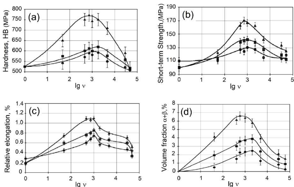
Fig. 1 - Dependence of hardness (a), short-term strength (b), relative elongation (c) and volume fraction of branched iron-containing phases ( \alpha + \beta ) on frequency for different values of density of electric current and content of Fe:
