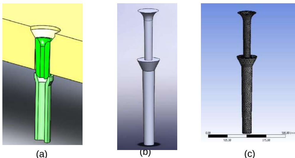
Fig. 1 – Schematic illustrations: 3-D model (a, b), grid for numerical simulations (c)
