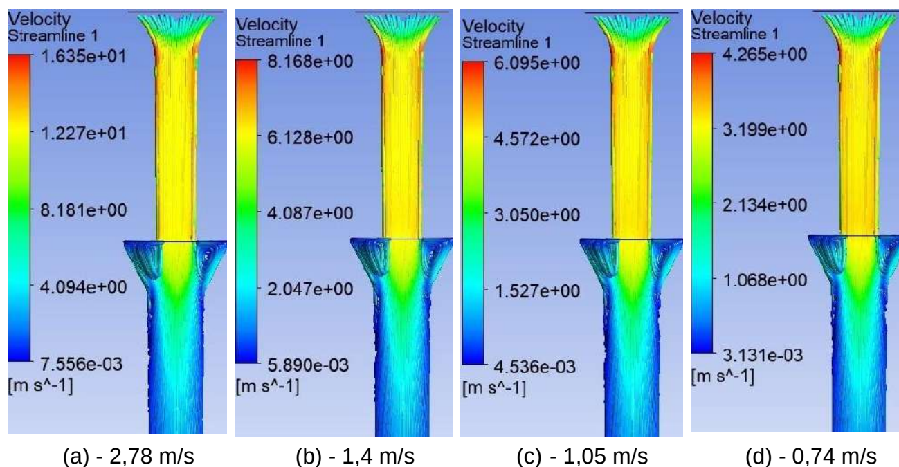
Fig. 2 – Numerical simulation of the pressure-and-flowrate characteristic with different linear casting speed ( \kappa - \epsilon turbulence model): during the pressure casting (a, b) and the low-pressure casting (c, d)
