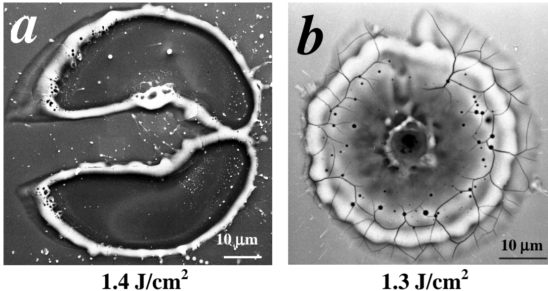
Fig. 3. SEM images of Sc/Si/10 MXM (a) and Sc/Si/33 MXM (b) after laser irradiation with fluences of \sim 1.4 and \sim 1.3 \text{J}/\text{cm}^2 , respectively.
