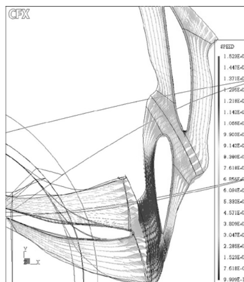
Fig. 2. The field of the vectors of the velocity of the spatial flow of fluid in the region of the stator columns, the blade guide vanes and runner in the optimal mode
