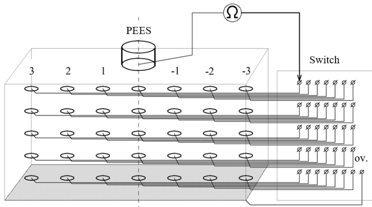
Fig. 6. Schematic of the laboratory installation to conduct the experiment
