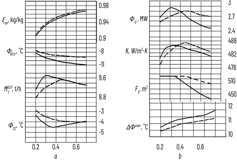
Fig. 1.8 Dependence of the efficiency indicators of the ARU evaporator on the change in pressure P_{MTP} (---- P_{MTP} = 0.29 MPa; - - - - P_{MTP} = 0.3 MPa) and the control action of the phlegm flow rate M_f : a – phlegm concentration \xi_\phi , refrigerant boiling temperature in the intertube space \Phi_{MTP} , refrigerant vapour flow rate at the evaporator outlet cooling temperature CG \Phi_{2C} ; b – cooling capacity \Phi_0 , heat transfer coefficient K , effective heat exchange surface F_X , mean logarithmic temperature difference \Delta\Phi^{CP} Source: [26]
