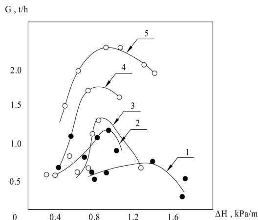
Fig. 7. Dependences of G (t/h) on the drop \Delta H (kPa/m) at R (MPa) [3]: 1 – 0.08; 2 – 0.14; 3 – 0.16; 4 – 0.2; 5 – 0.27
