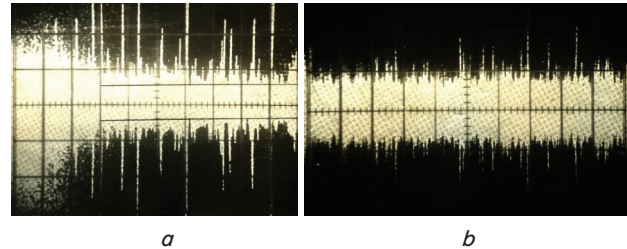
Fig. 9. Change in the spectra of the AcE amplitudes under different jet states: a – unloading; G = 1.5 \dots 1.7 \text{ t/h} ; H = 0 \dots -5 \text{ mmH}_2\text{O} ; b – overload (blockage); G = 0.9 \dots 1 \text{ t/h} ; H = +20 \text{ mmH}_2\text{O}
