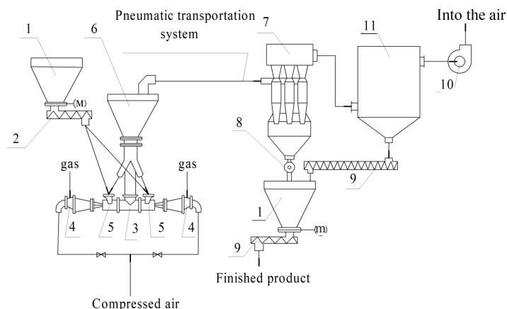
Fig. 3. An industrial gas-jet plant scheme (VMMP):
