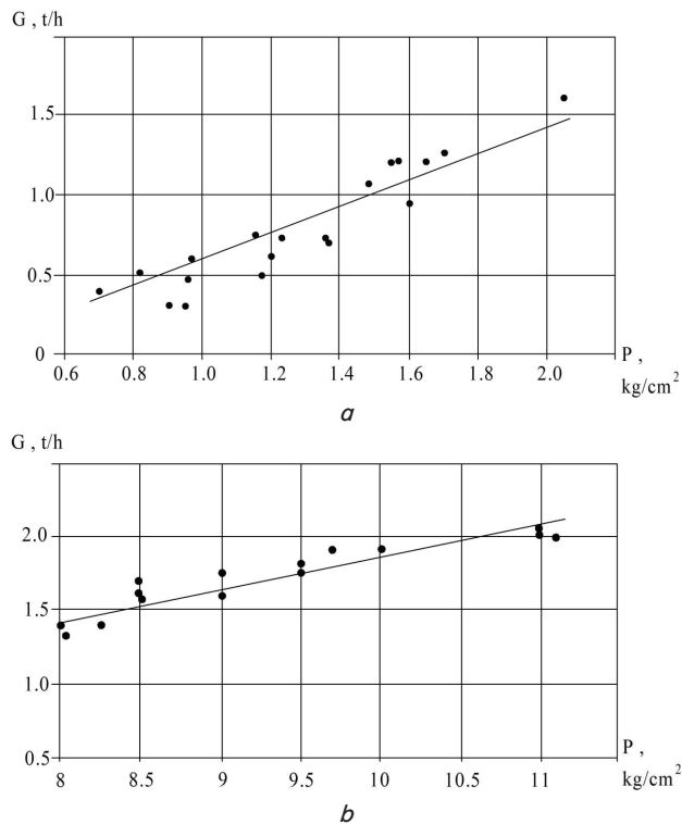
Fig. 6. The impact of the energy carrier pressure on performance G : a – natural gas combustion products; T=400...600 °C; b – overheated steam; T=200...230 °C
