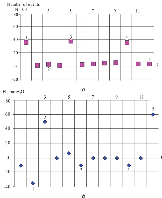
Fig. 8. Time-dependent change in acoustic radiation N and static pressure H : a – a change in the acoustic radiation N(t) ; b – a change in the static pressure H(t)
