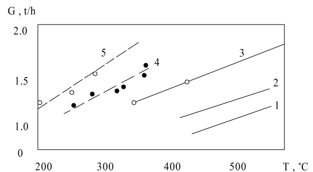
Fig. 5. Effect of the energy carrier temperature on the performance of a gas-jet (1, 2, 3) and steam-jet (4, 5) mills: pressure P (MPa): 1 – 0.15; 2 – 0.18; 3 – 0.27; 4 – 0.9; 5 – 1.1
