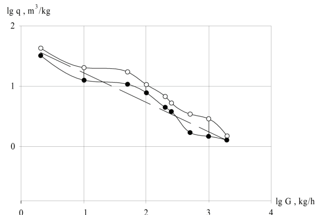
Fig. 1. Dependence of the specific energy carrier consumption on the performance of a jet unit: o – maximal; • – minimal; – – the estimation value
