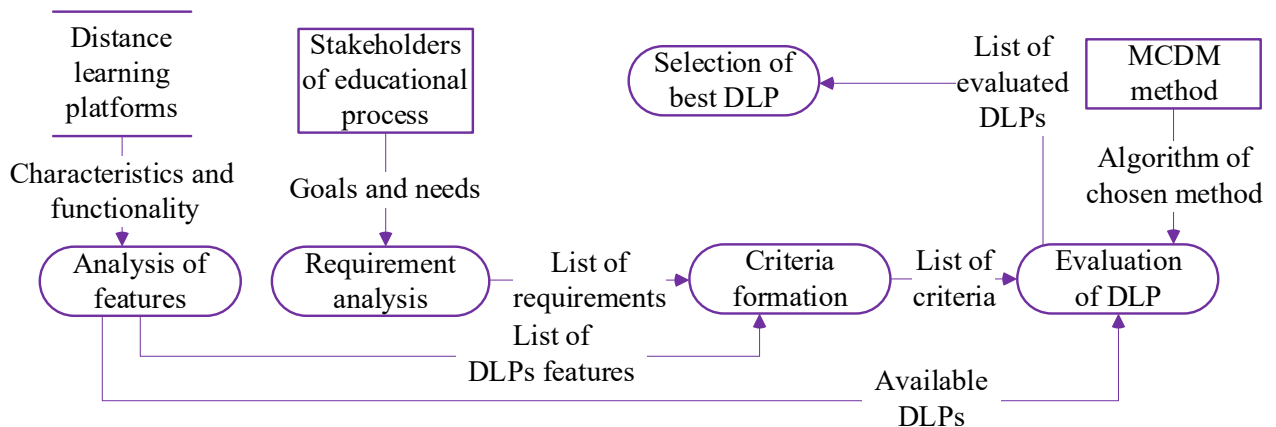
Figure 1 – Data flow diagram of selection process of DLP
