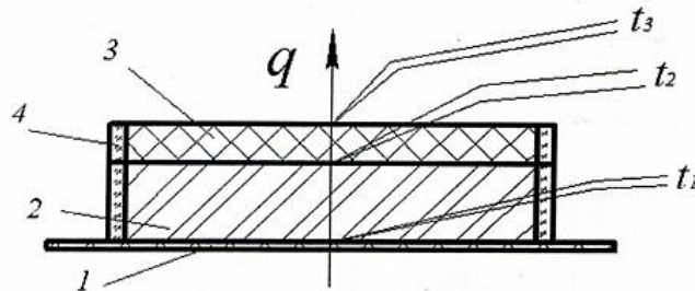
Fig. 1 – Schematic diagram of the of the thermal conductivity coefficient measuring method
